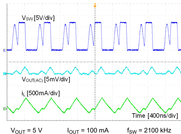
Figure 8-3. DCM Mode
