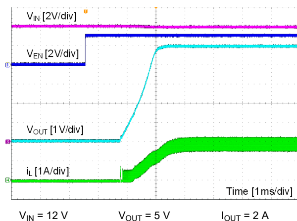
Figure 8-7. Start-Up by EN
