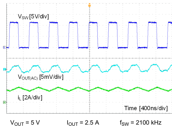
Figure 8-2. CCM Mode
