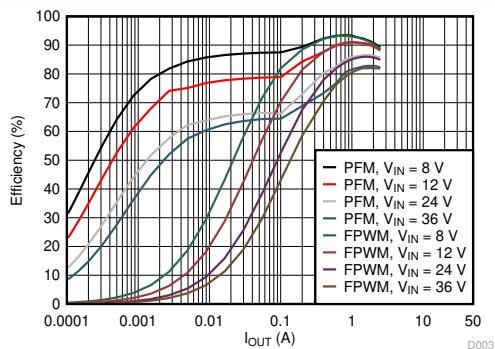
Figure 6-1. Efficiency vs Load Current
