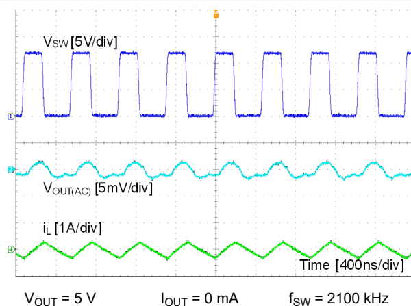
Figure 8-5. FPWM Mode
