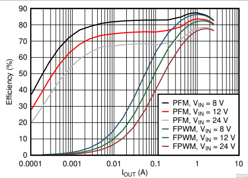
Figure 6-2. Efficiency vs Load Current
