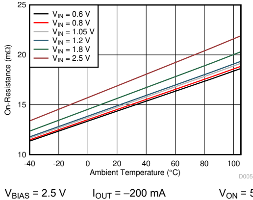
Figure 7-7. On-Resistance vs Ambient Temperature Single Channel
