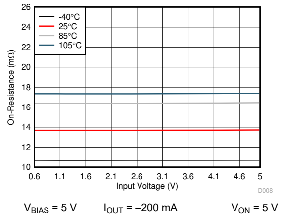
Figure 7-10. On-Resistance vs Input Voltage Single Channel - Across Ambient Temperatures
