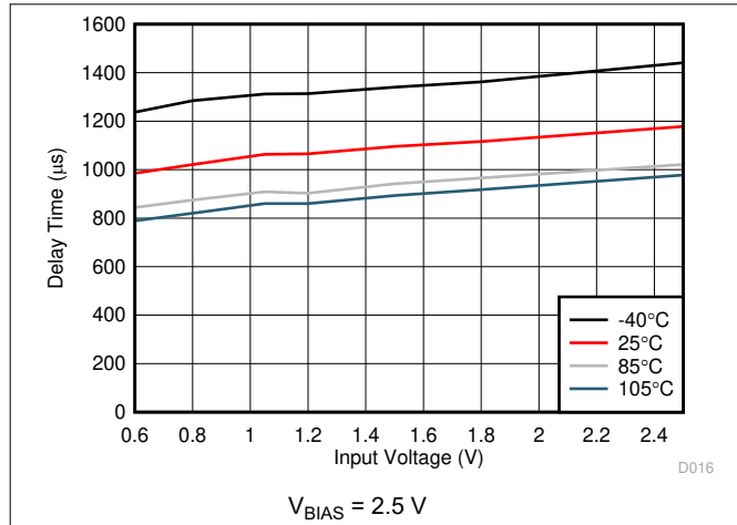
Figure 7-16. Delay Time vs Input Voltage
