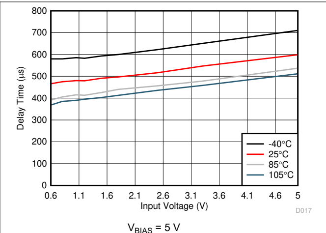
Figure 7-17. Delay Time vs Input Voltage
