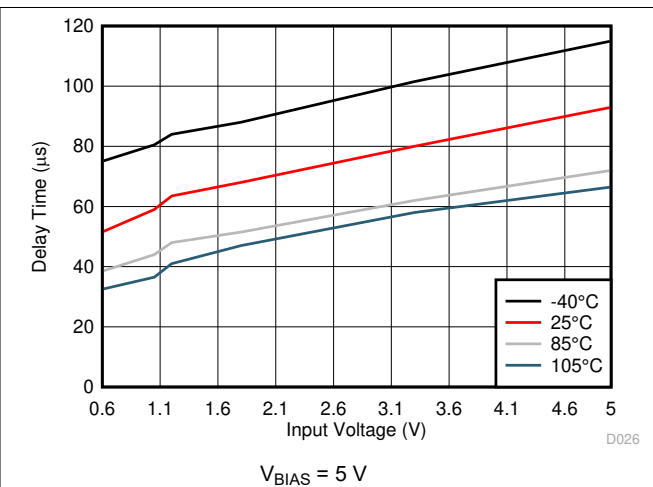
Figure 7-35. Delay Time vs Input Voltage
