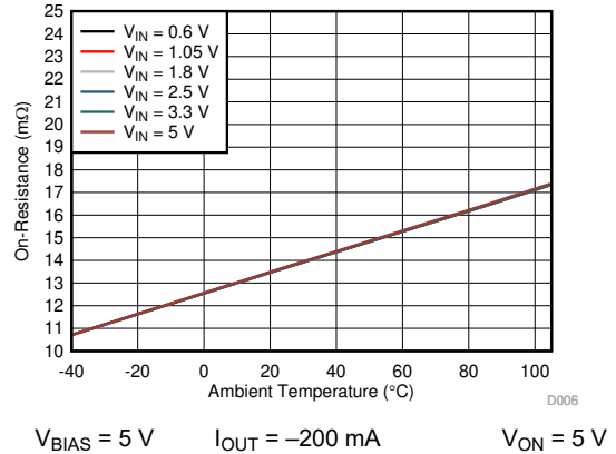
Figure 7-8. On-Resistance vs Ambient Temperature Single Channel
