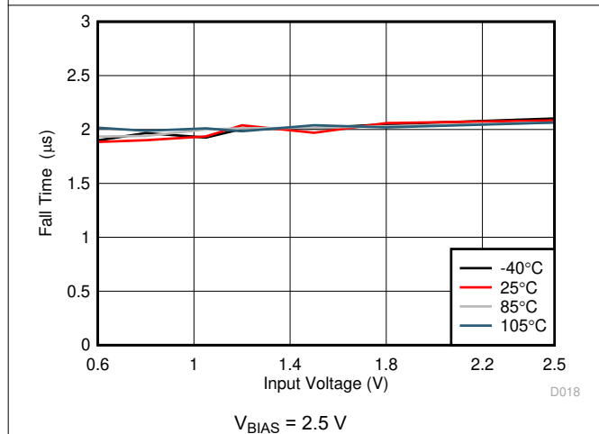
Figure 7-18. Fall Time vs Input Voltage
