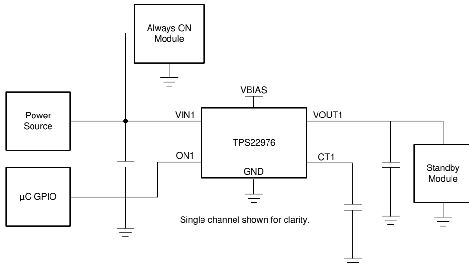
Figure 10-2. Standby Power Reduction
