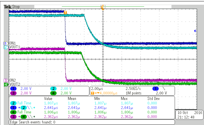
Figure 7-33. Turnoff Response Time
