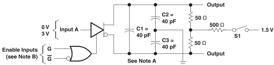
TEST CIRCUIT
